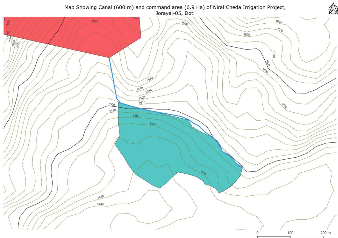
Figure 1-1 Contour map of Niral Cheda irrigation project
